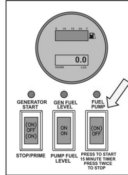
Typical Fuel Pump Switch Locations on the Command Center
