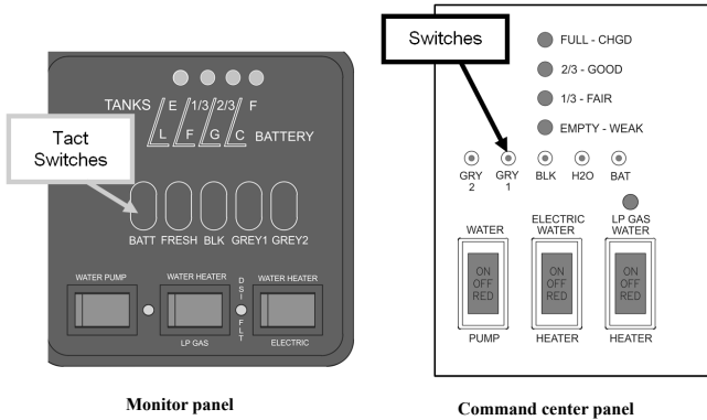
Command center panel
