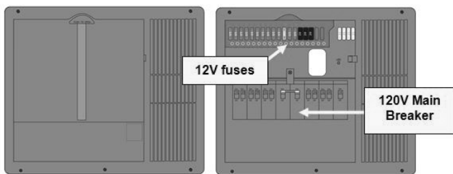
50A Load Center Panel w/120 volt Main breaker
