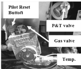
Water Heater pilot ignition
